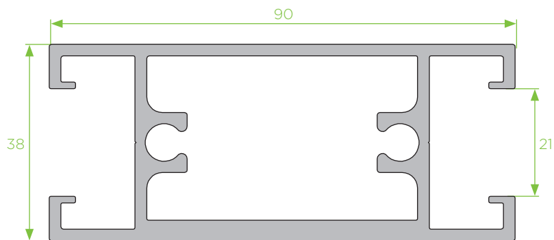
PT - 33 travessa central
