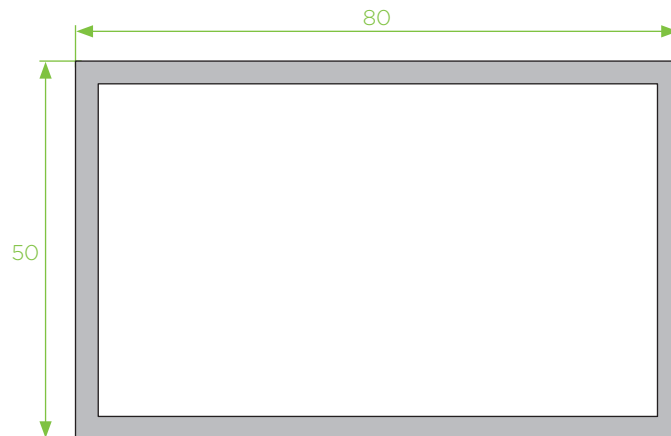
80x50x3,0 tubo retangular
