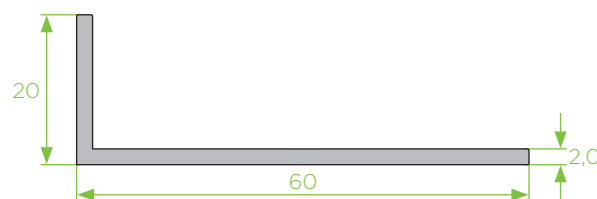
P - 50 cantoneira
