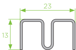
P - 31 padieira
