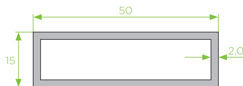
50x15x2,0 tubo retangular
