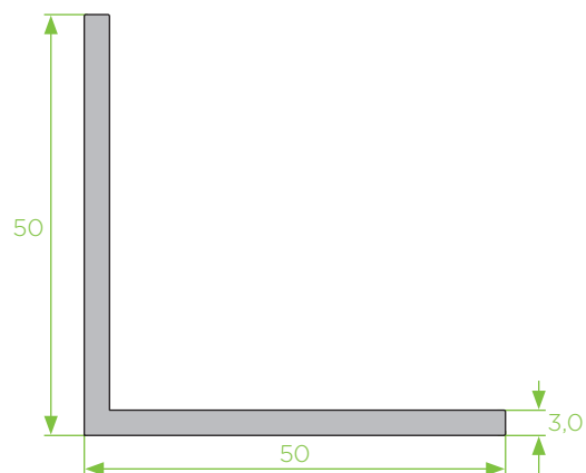
P - 15 cantoneira
