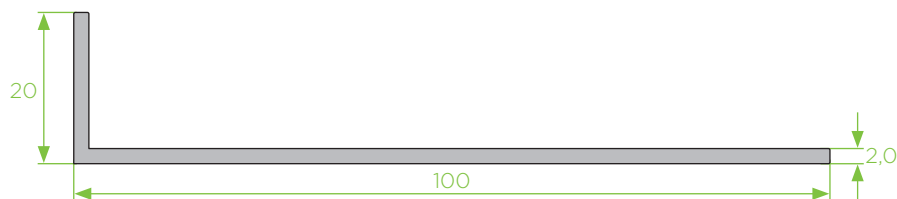
P - 52 cantoneira
