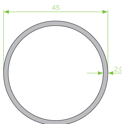
45x2,0 tubo redondo
