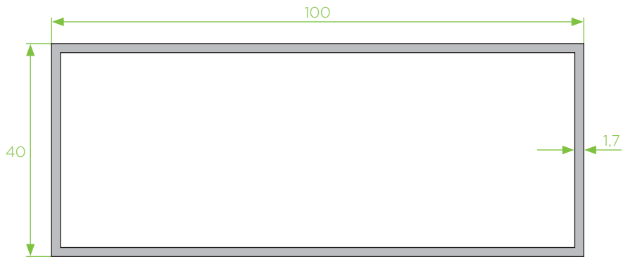
100x40x1,7 tubo retangular
