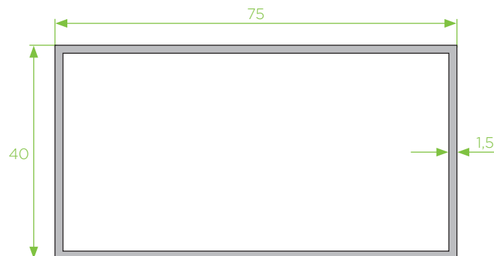
75x40x1,5 tubo retangular
