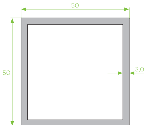
PT - 50 tubo quadrado 50x50x3,0
