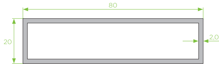
80x20x2,0 tubo retangular
